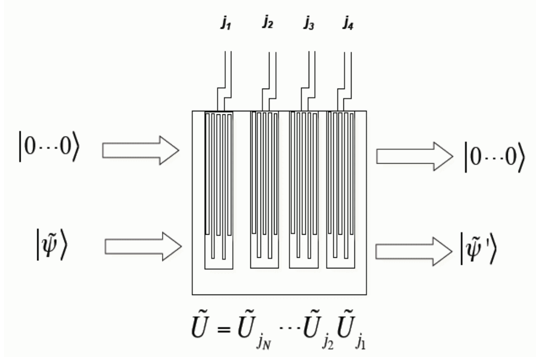
Fig. 2: Decomposition of unitary evolution into a series of unitary gates each generated by one-sparse Hamiltonians.
