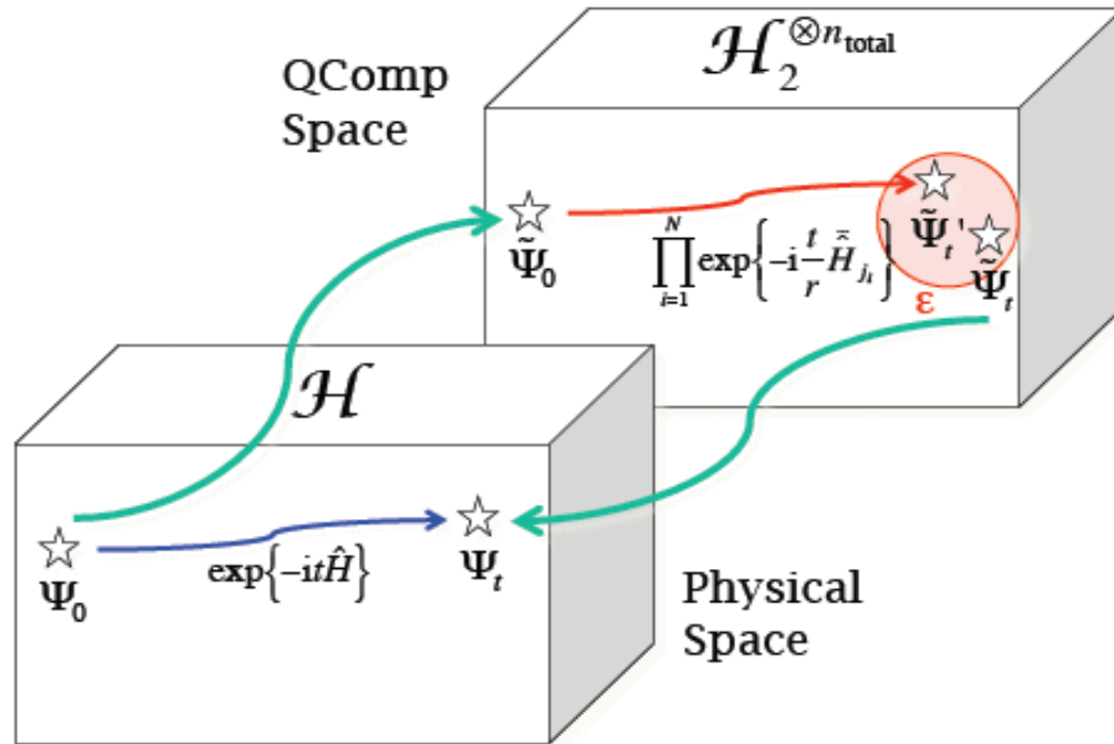
FIG. 1: Simulating Hamiltonian evolution in a physical space on a quantum computer.
