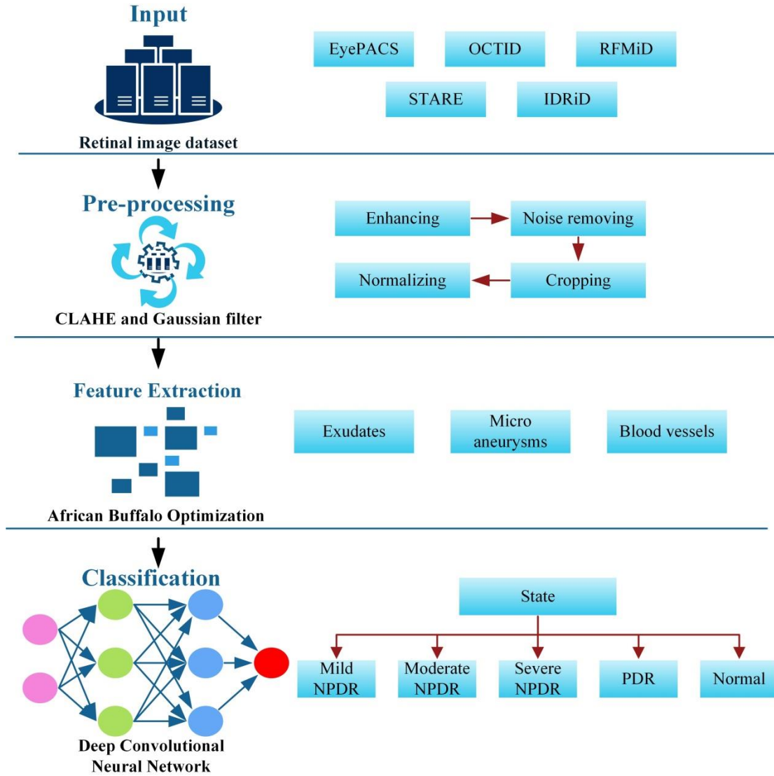
Fig.2: Processing phases of proposed AB-DCNN model
