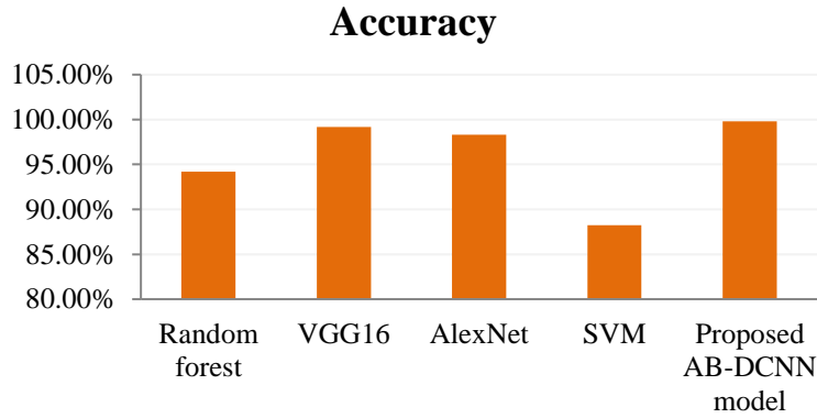
Fig 4: Comparison of Accuracy
