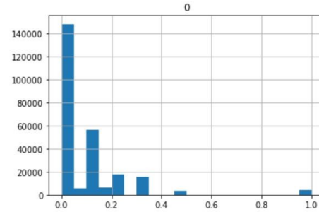
Figure 7. After normalization
