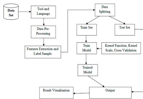
Figure 1. Research Framework
