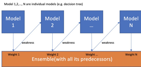
Figure 8. Boosting
