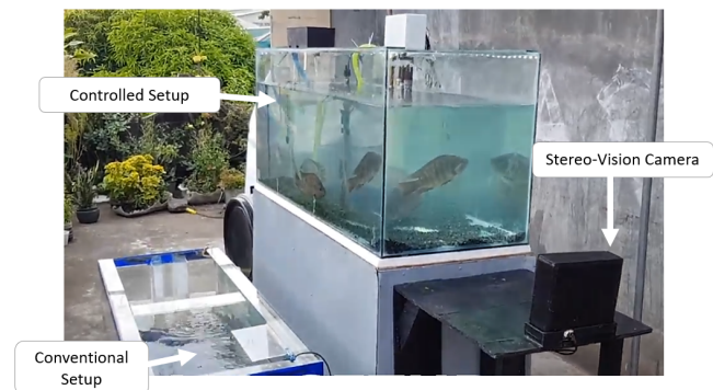
Figure 2. Conventional and Controlled Aquaculture System Setups
