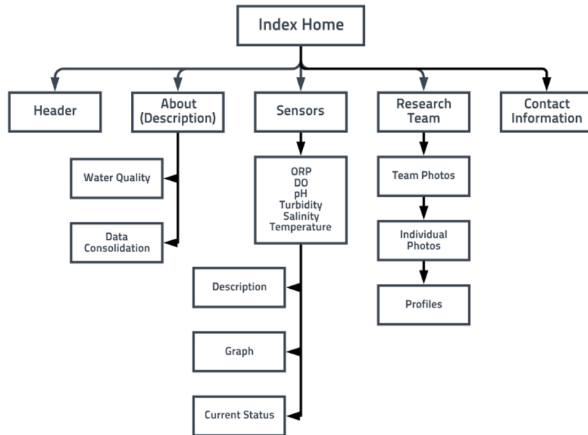
Figure 4. Web Application Structure Diagram
