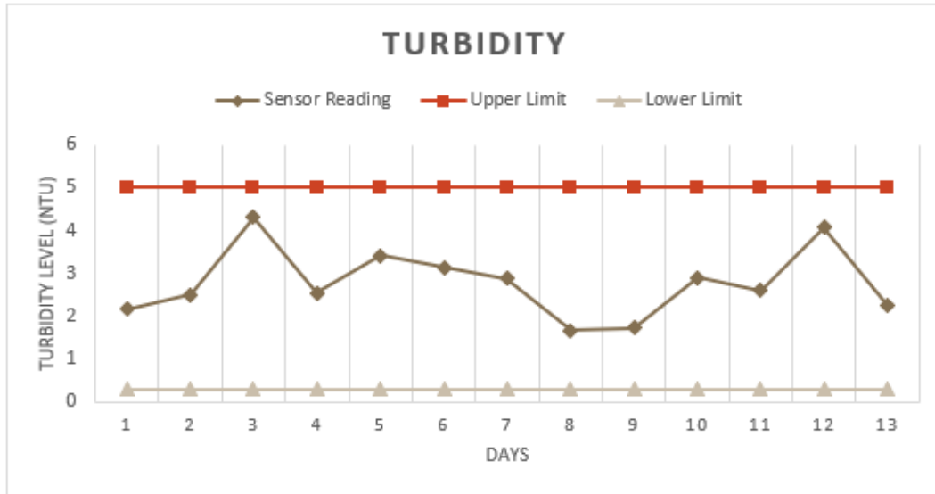
Figure 6. Turbidity Sensor Readings with Correction Response
