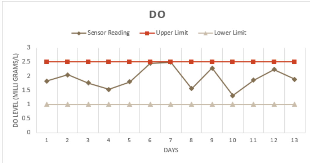
Figure 10. Dissolved Oxygen Sensor Readings with Correction Response
