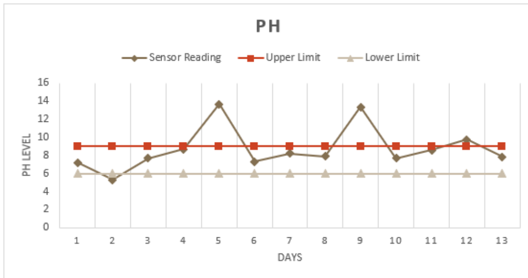
Figure 5. Potential Hydrogen (pH) Sensor Readings with Correction Response
