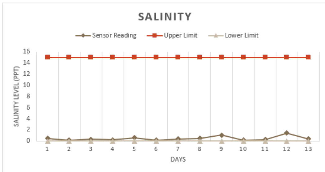
Figure 9. Salinity Sensor Readings with Correction Response
