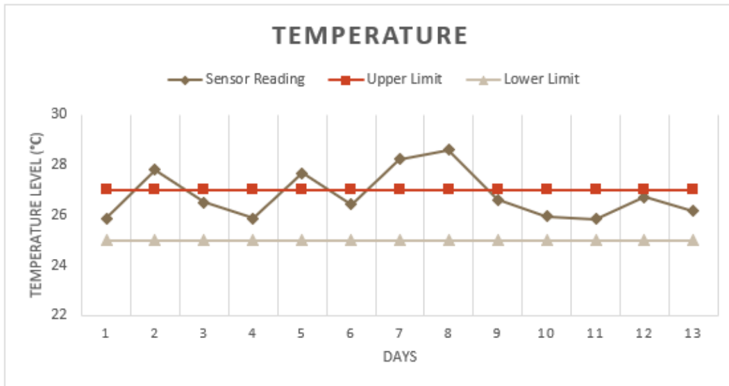
Figure 8. Temperature Sensor Readings with Correction Response
