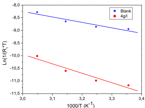
Figure 7 Variation of \text{Ln}(1/(R_t \times T)) versus 10^3/T for blank and 0.5 M H 2 SO 4 + 4 g/l of CAE.
