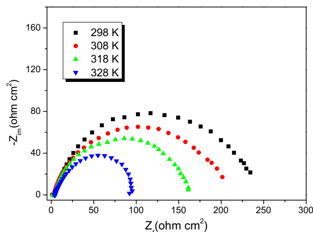
Figure 5 Nyquist plots for corrosion of steel in 0.5 M H 2 SO 4 + 4 g/l CAE at different temperatures.
