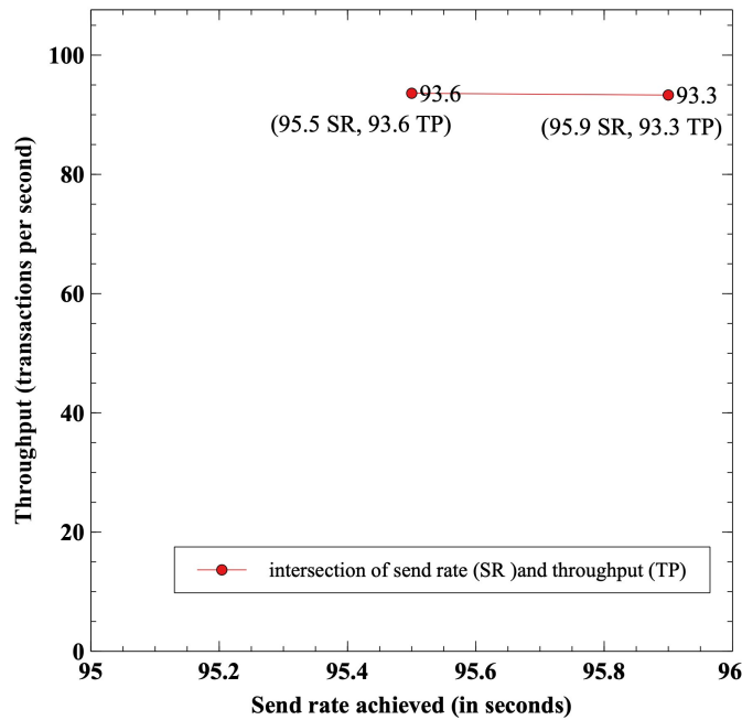
Figure 8. Transaction throughput
