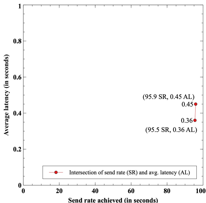
Figure 7. Transaction latency
