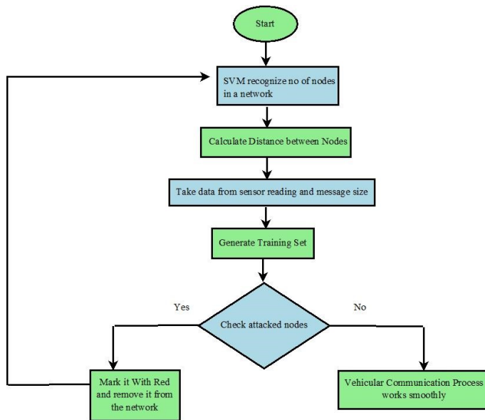
Figure 1. SVM for DOS detection
