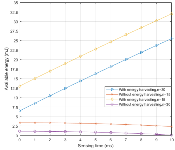
Figure 9. Available energy per node versus sensing time
