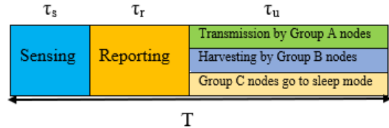
Figure 2. Cooperative spectrum detection and data transmission with energy harvesting frame structure
