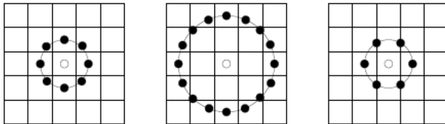
Figure 3. Circular neighborhoods: (8, 1) , (16, 2) and (6, 1)
