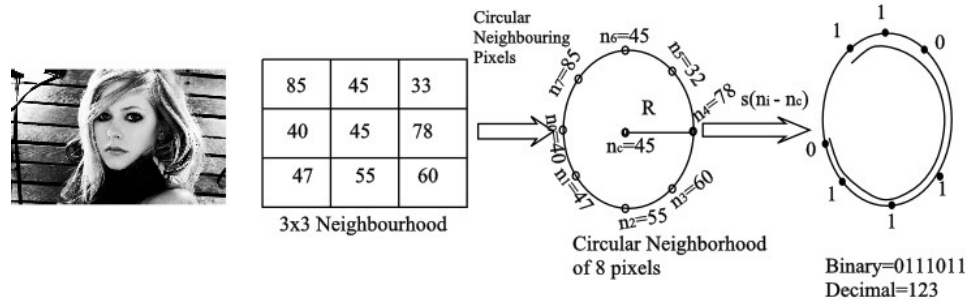
Figure 2. Central pixel and its n circularly neighbors with radius R
