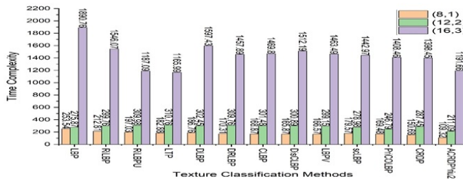
Figure 26. Time complexity computation using 2D HeLa
