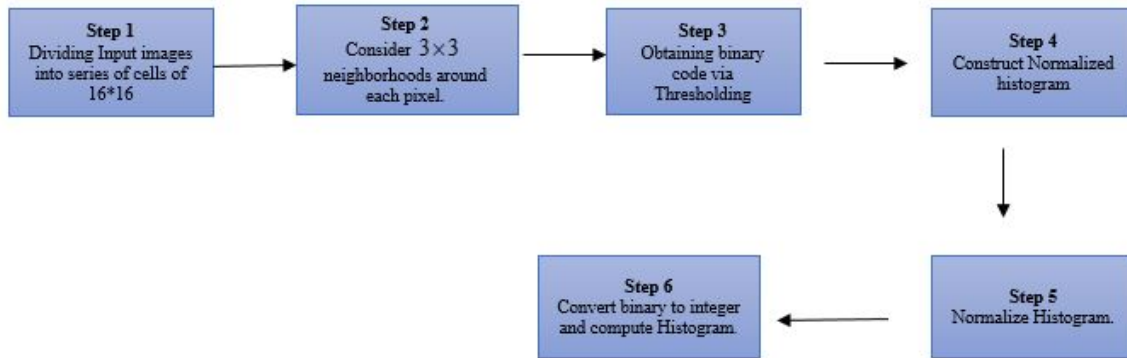
Figure 4. Pipeline to extract LBP like features
