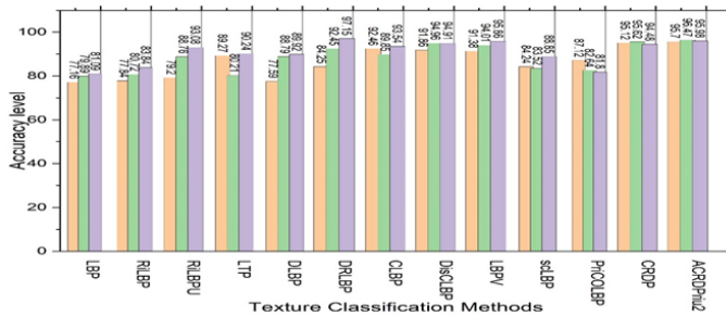
Figure 25. Classification accuracy using Chi-Square distance on KIMIA PATH 960
