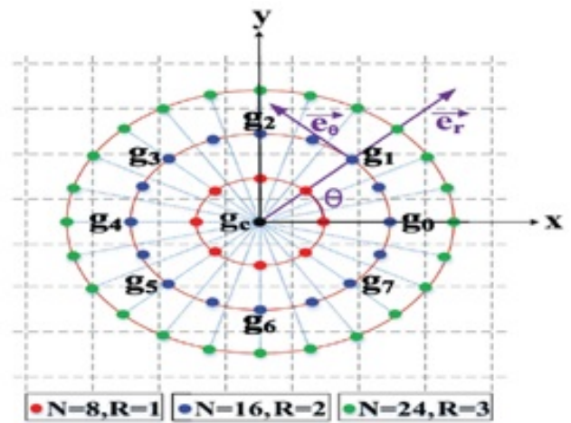
Figure 5. Circular Symmetric Neighborhood for Distinct (N,R) Values
