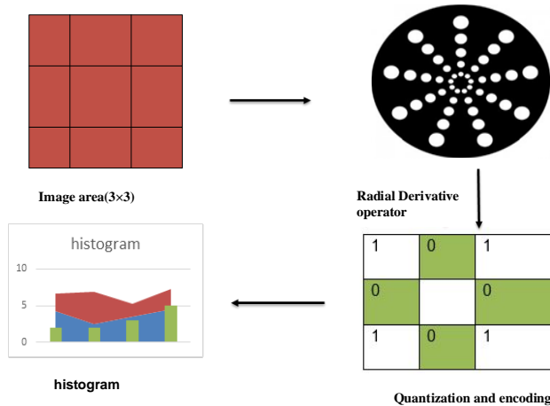
Figure 9. Radial derivative operator
