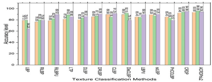
Figure 23. Classification accuracy using L 2 -norm distance on 2D Hela
