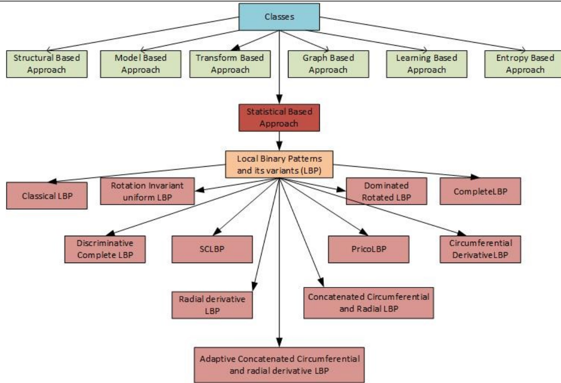
Figure 1. Detailed list of texture methods)
