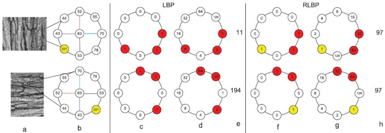
Figure 6. The effect of rotation on LBP and RLBP operator
