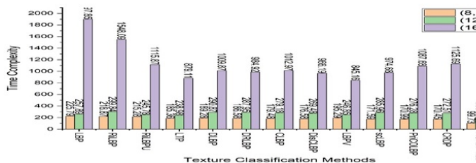
Figure 27. Time complexity computation using KIMIA PATH 960
