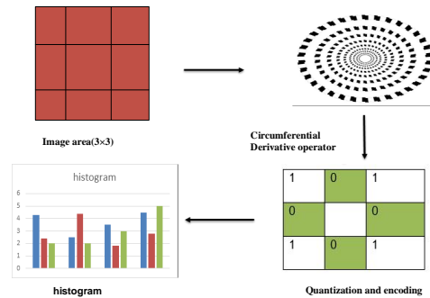
Figure 8. Circumferential Derivative Pattern Operator
