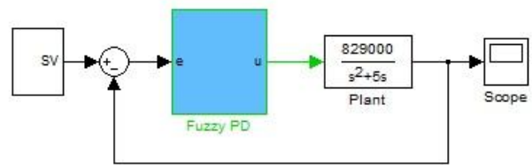
Figure 5. Simulink model of HEV with Fuzzy PD controller
