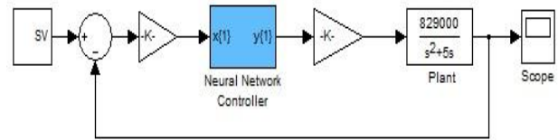
Figure 10. Simulink model of HEV with ANN controller
