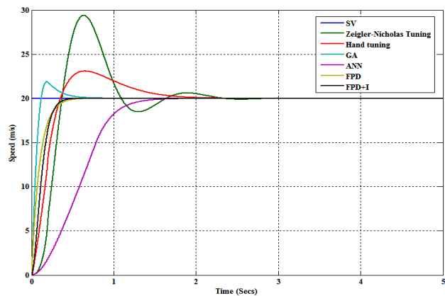
Figure 17. Combined Vehicle Response
